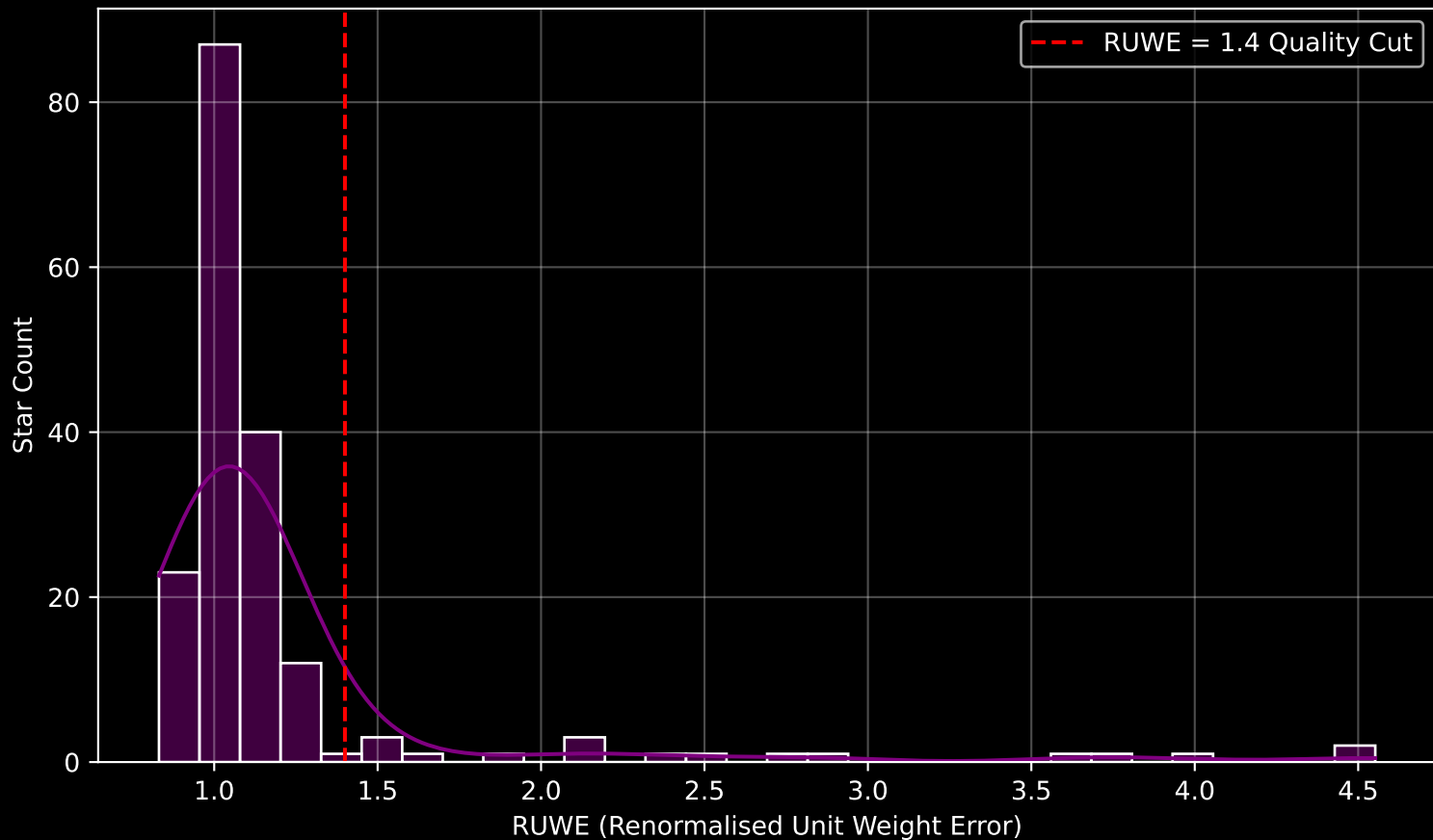
GAPOGEE DR17 Field [173+18] RUWE Distribution (n= 180)
