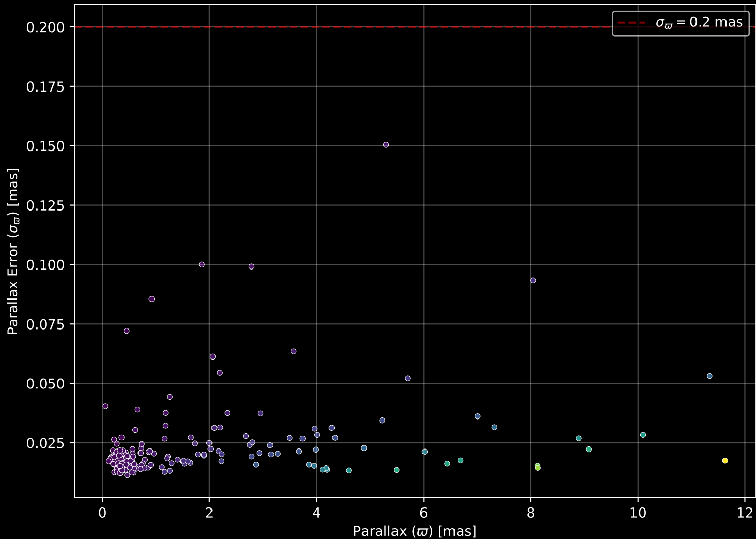
APOGEE DR17 Field: [173+18] Parallax Quality (n= 181)
