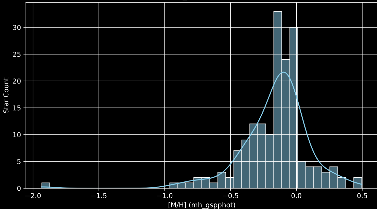
APOGEE DR17 Field: [173+18 [M/H] (mh_gspphot) (n= 175)
