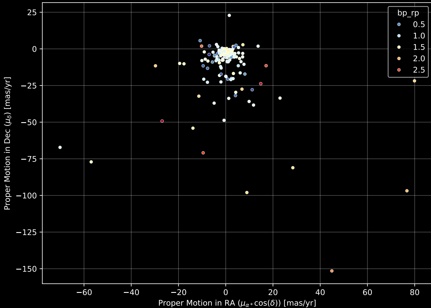
APOGEE DR17 Field: [173+18] Proper Motion Diagram (n= 181)
