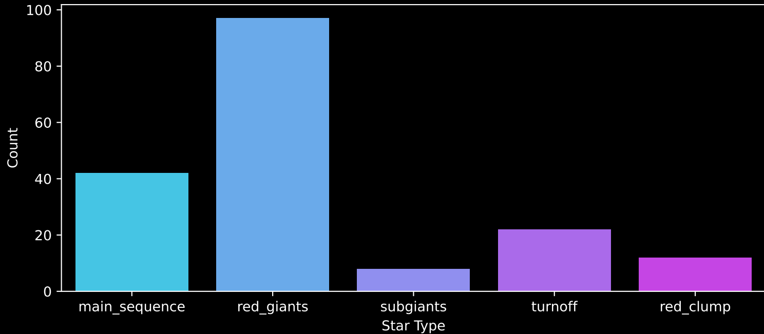
APOGEE DR17 Field: [173+18] Count plot of Star Type
